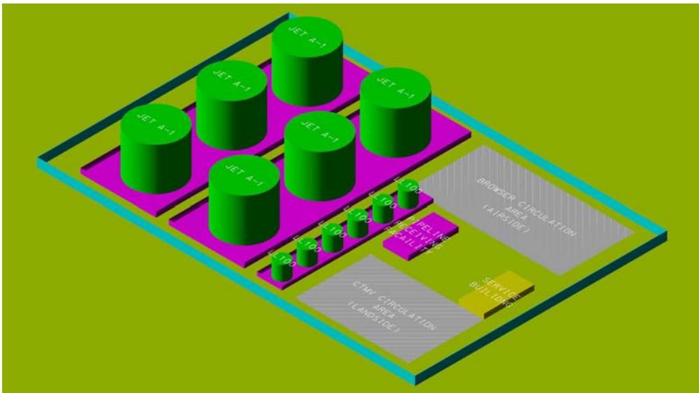
airport fuel farm for Jet A-1 and avgas
